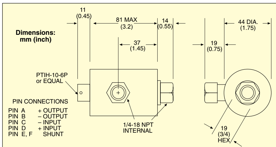
STANDARD PX81D1-100D5T, shown than size.
