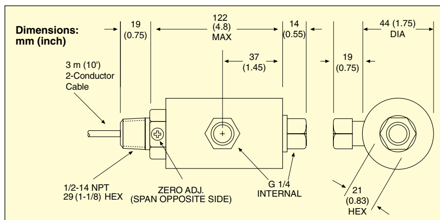
METRIC PXM81MD0-1.40BARDI , shown smaller than actual size.
