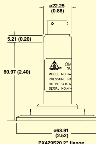
PX429S20 2" flange
