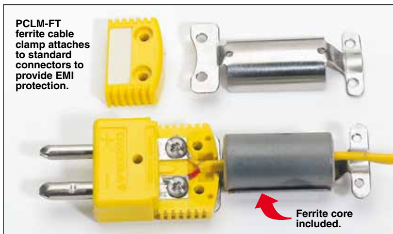
PCLM-FT ferrite core and cable clamp, standard size.
