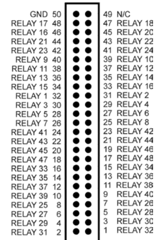
50 PIN CONNECTOR ON CIO-ERB48
