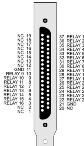
37 PIN CONNECTOR ON CIO-ERB24
