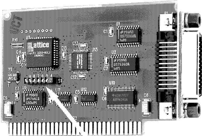
Address Switch
