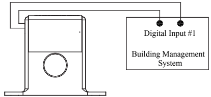
FIGURE 5: DIGITAL CIRCUIT
