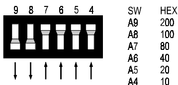
BASE ADDRESS SWITCH - Address 300H shown here.
