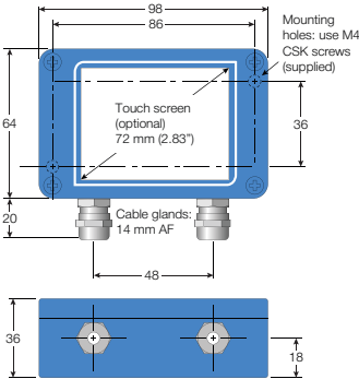
Electronics Module
