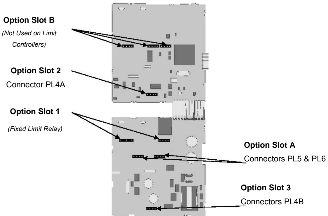
Figure 8. Option Module Connectors - \frac{1}{8} & \frac{1}{4} DIN Instruments
