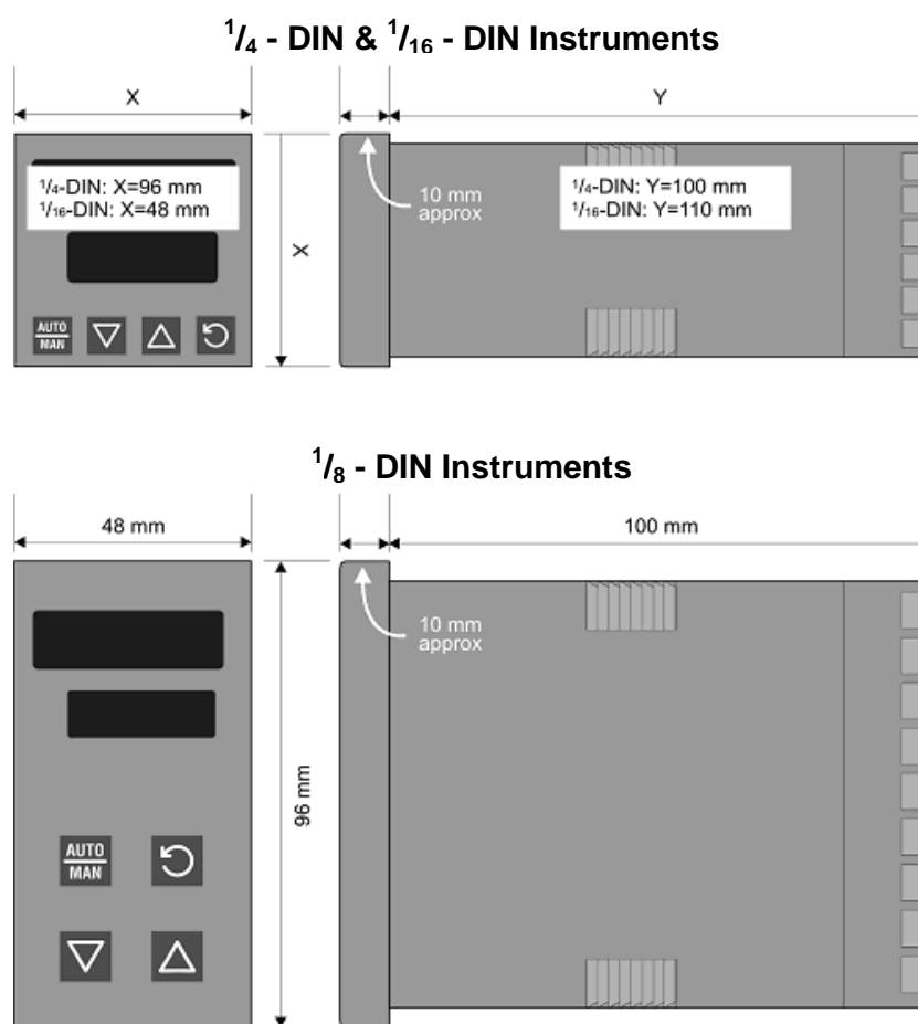
Figure 1. Main dimensions
