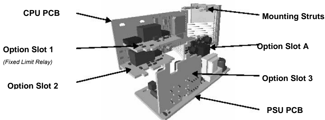
Figure 5. Location of Option Slots - \frac{1}{16} DIN Instruments
