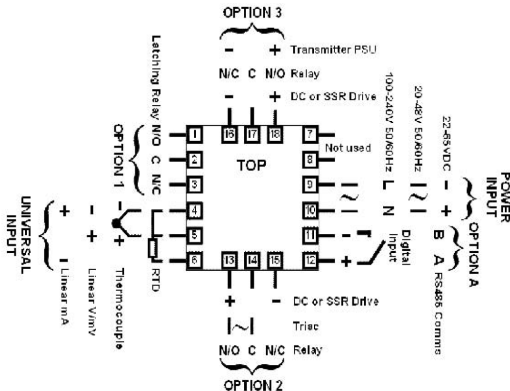
Figure 11. Rear terminals ( \frac{1}{16} -DIN Instruments)
