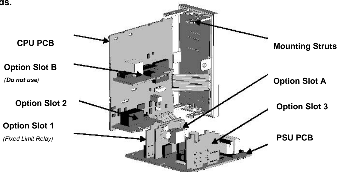
Figure 6. Location of Option Slots - \frac{1}{8} & \frac{1}{4} DIN Instruments
