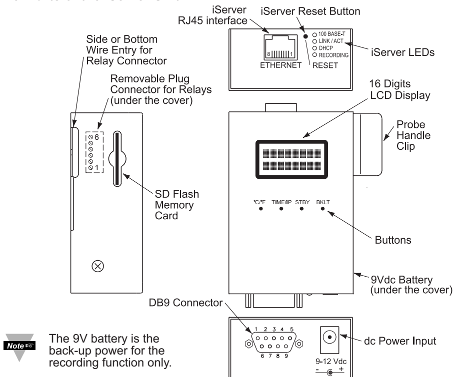
Figure 2.3 Parts of the iServer Unit
