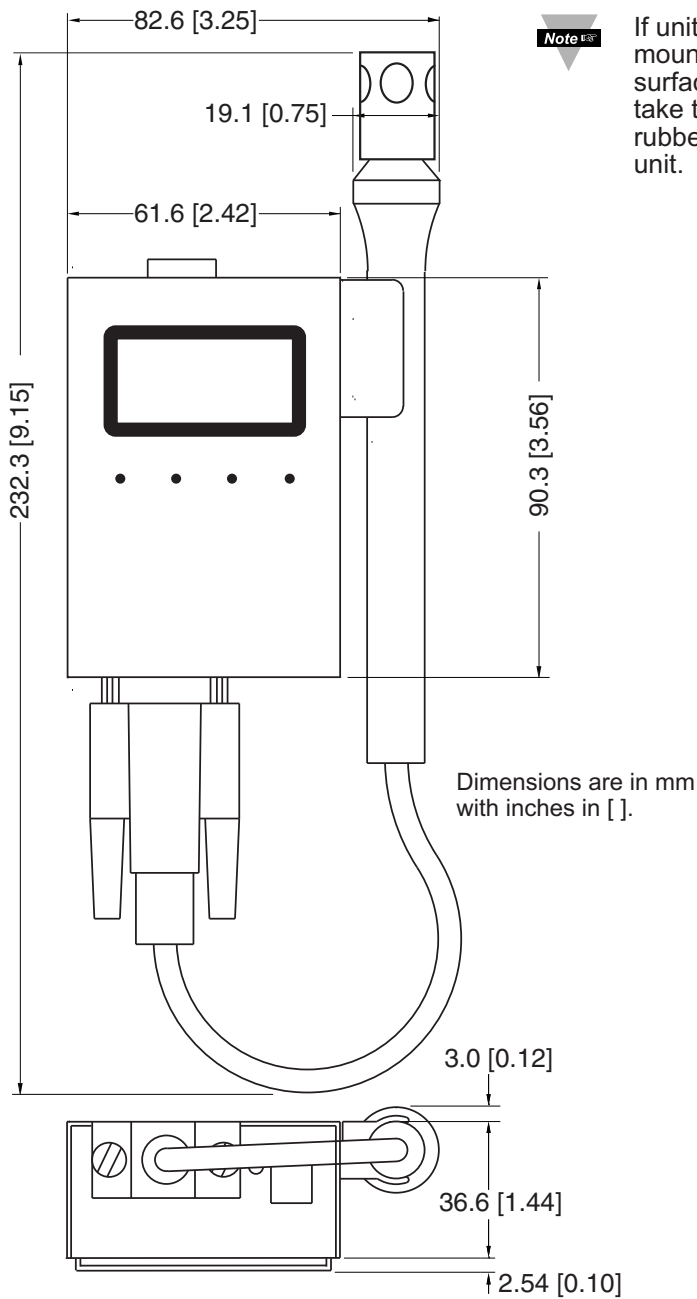
Figure 2.1 Dimensions
