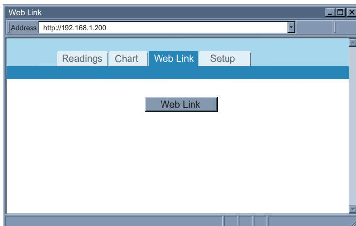
Figure 4.35 Web Link
