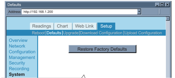
Figure 4.27 System: Defaults
