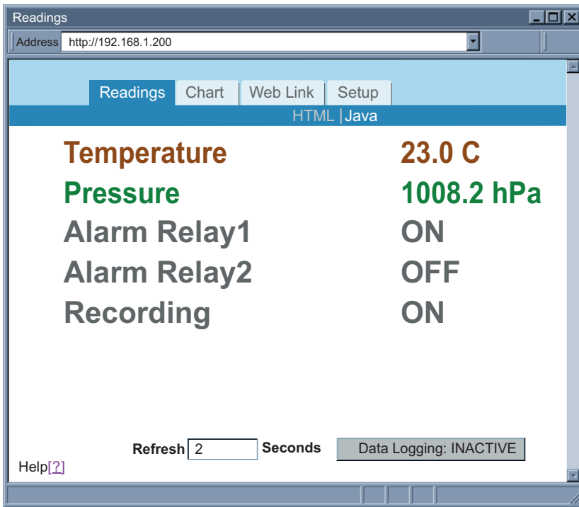
Figure 4.33 Readings: Java
