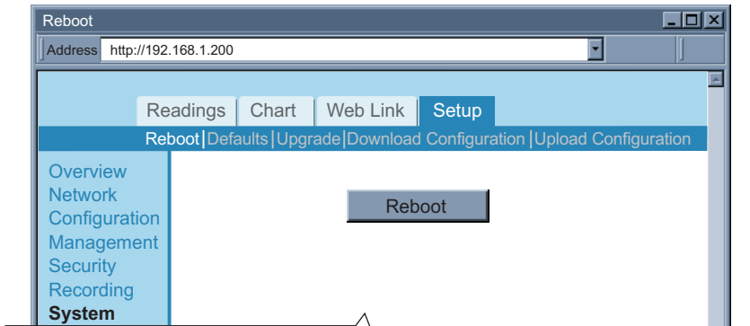
Figure 4.26 System: Reboot
