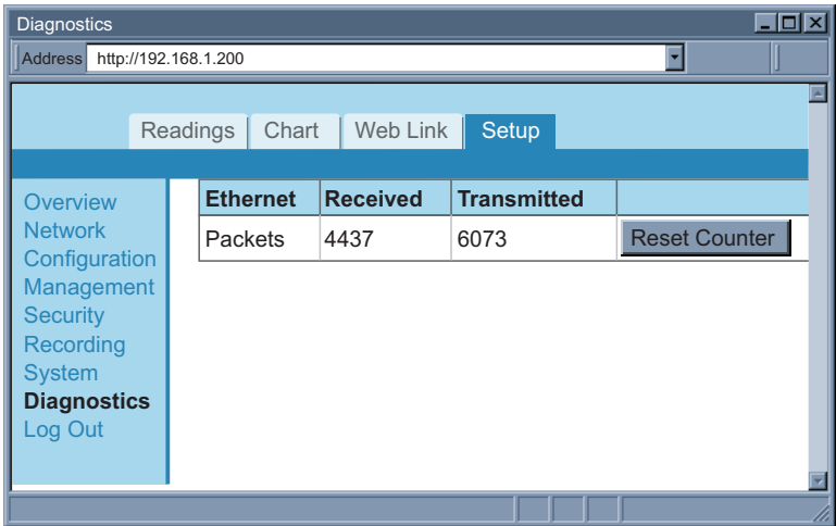
Figure 4.31 Diagnostics
