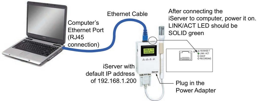
Figure 4.2 Connecting Computer Directly to iServer
