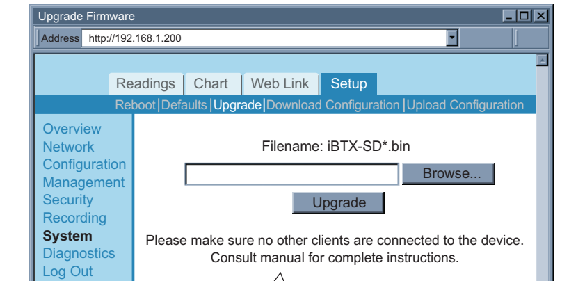
Figure 4.28 System: Upgrade
