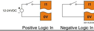
Positive Logic In
