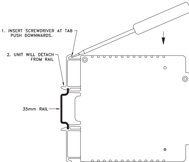
Figure 2.4a Mounting - Installation
