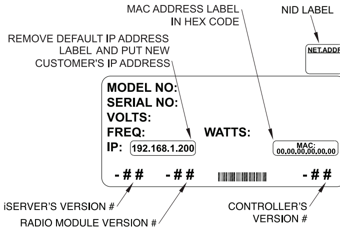
Figure 3.1 Label Detail
