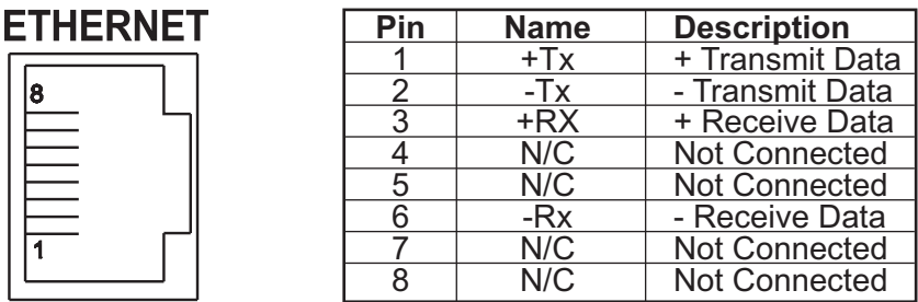
Figure 2.11 RJ45
