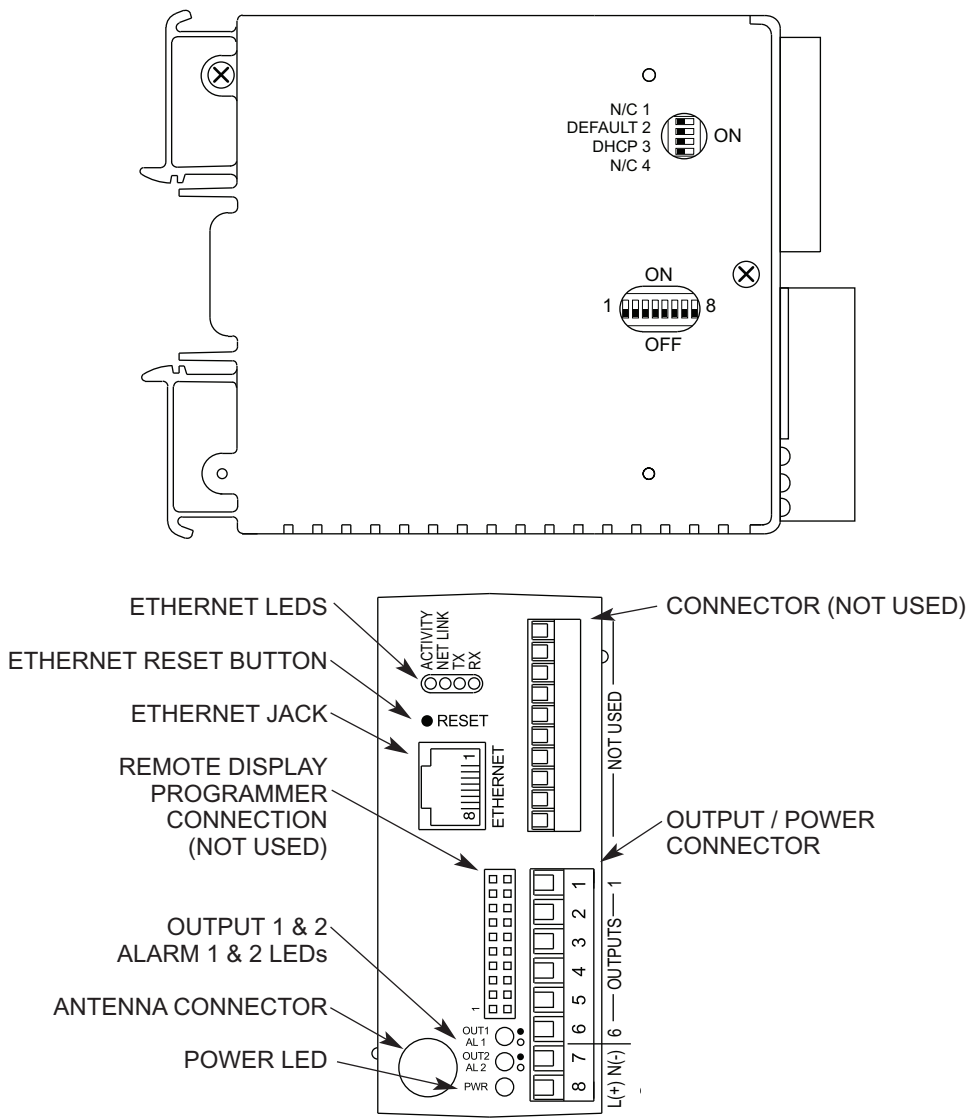
Figure 2.1 Front and Side Views
