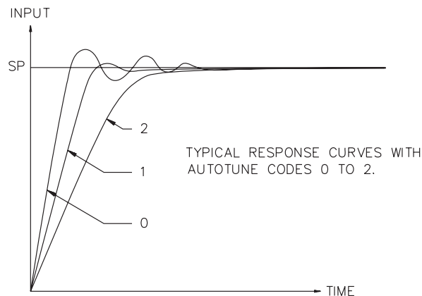
Figure 15, Auto-Tune Code
