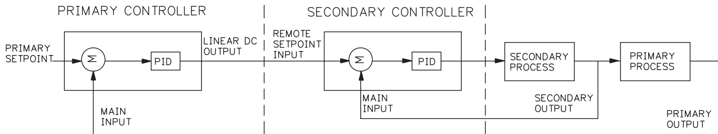
Figure 34, Cascade Control
