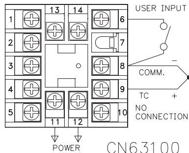
Figure 4, Thermocouple Connection
