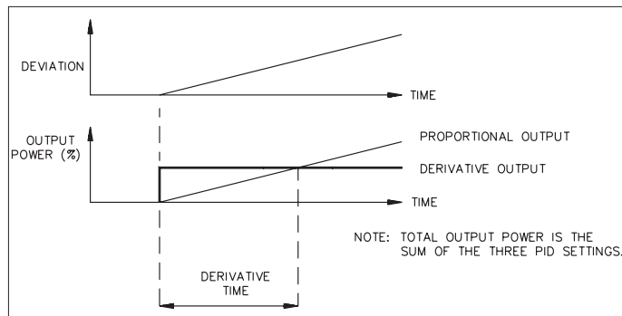
Figure 31, Derivative Time
