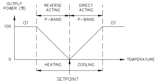
Figure 29, Proportional Band
