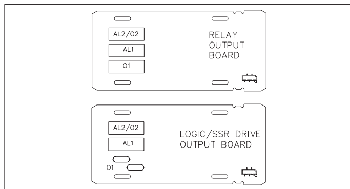
Figure 40, Output Boards
