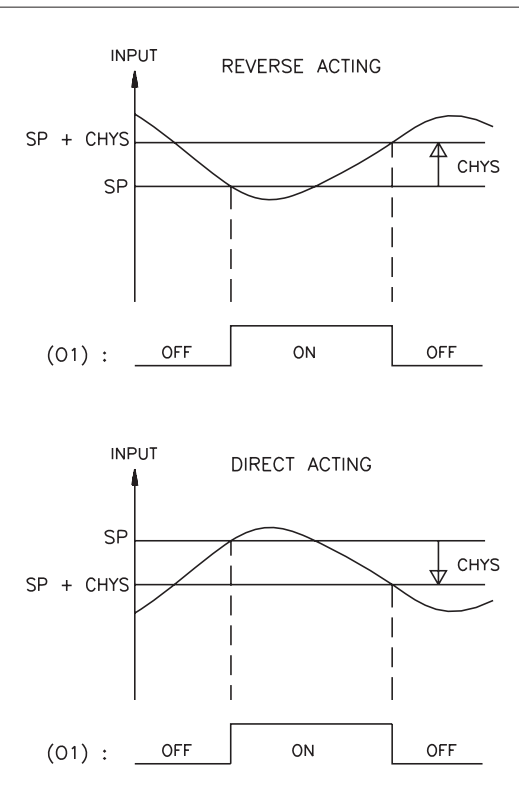
Figure 22, Output 1 (O1) ON/OFF Control Software Revision V3.x or Earlier
