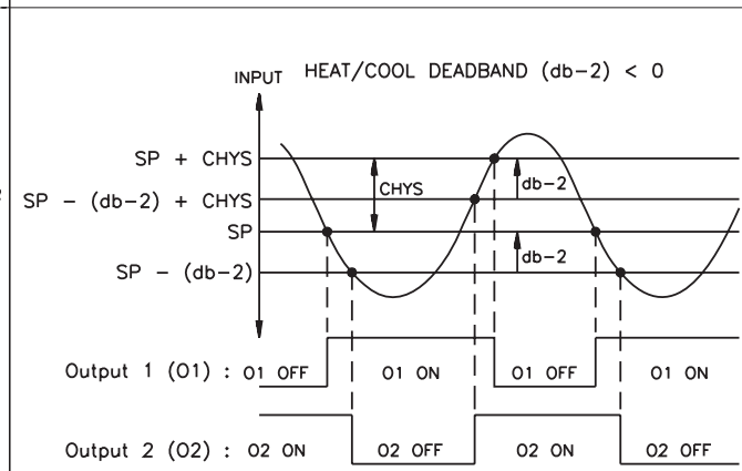
Figure 26, O1/O2 ON/OFF Control Software Revisions V3.x or Earlier
