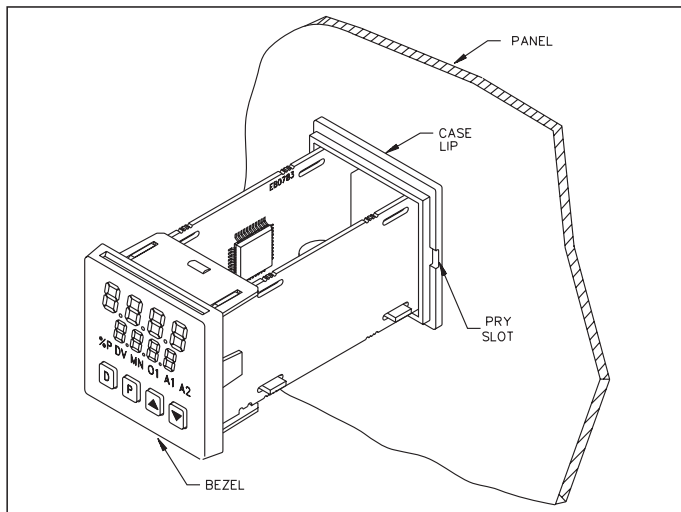
Figure 3, Bezel Assembly
