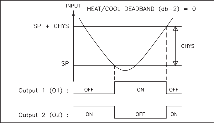
Figure 24, O1/O2 ON/OFF Control Software Revisions V3.x or Earlier
