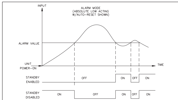
Figure 17, Alarm Standby Delay Sequence
