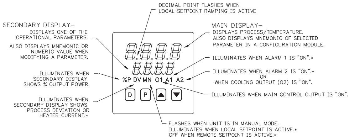
Figure 11, Front Panel
