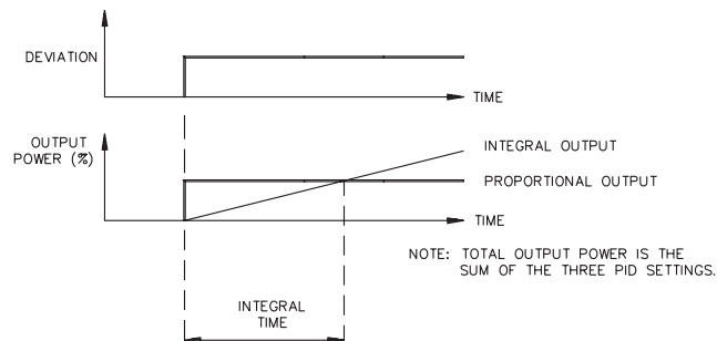
Figure 30, Integral Time
