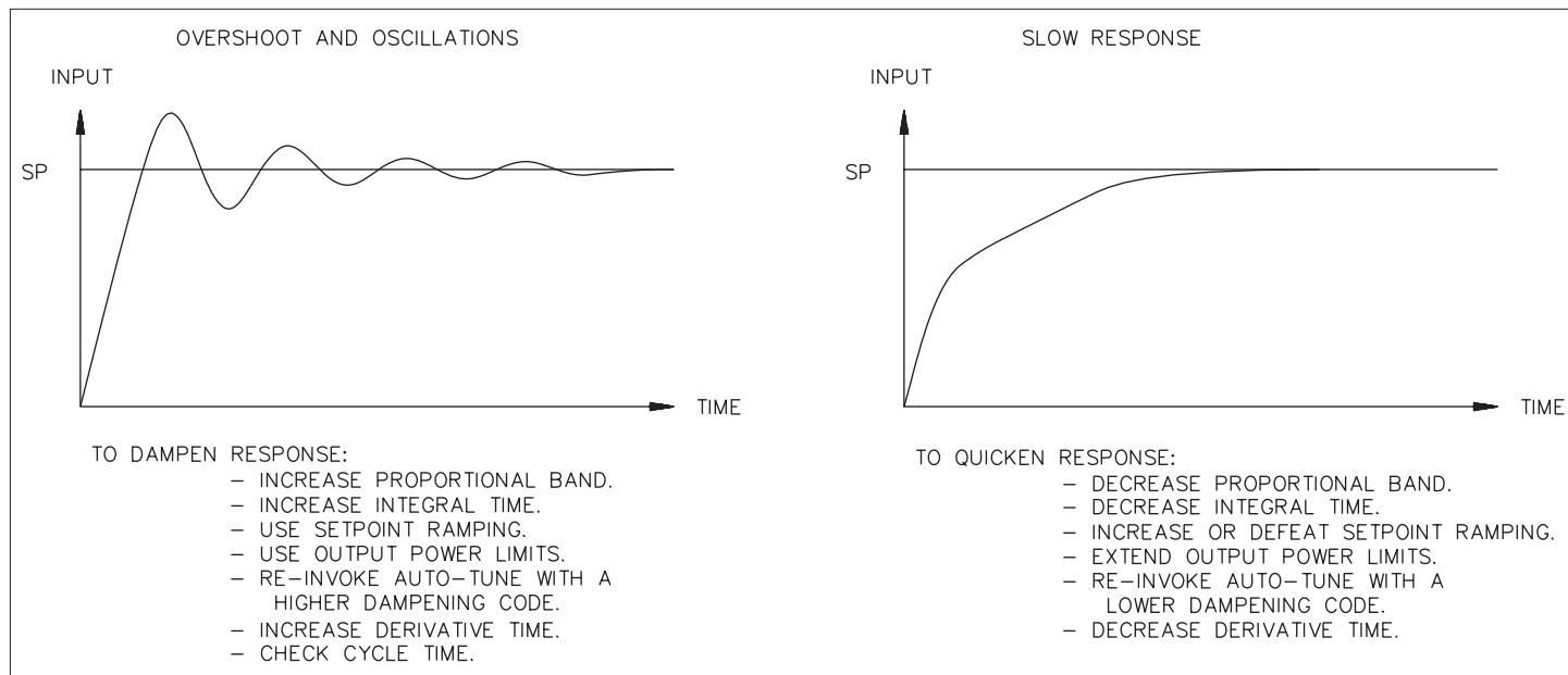
Figure 33, Process Response Extremes
