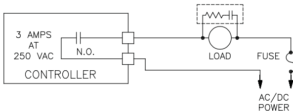
Figure 7, Relay Output
