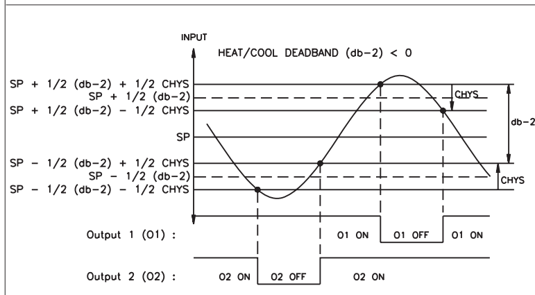
Figure 25, O1/O2 ON/OFF Control Software Revision V4.0 or Later
