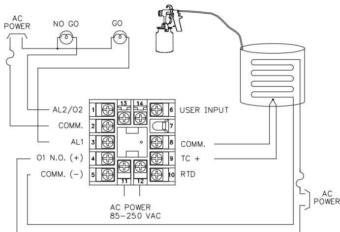
Figure 37, OEM Paint Sprayer Application
