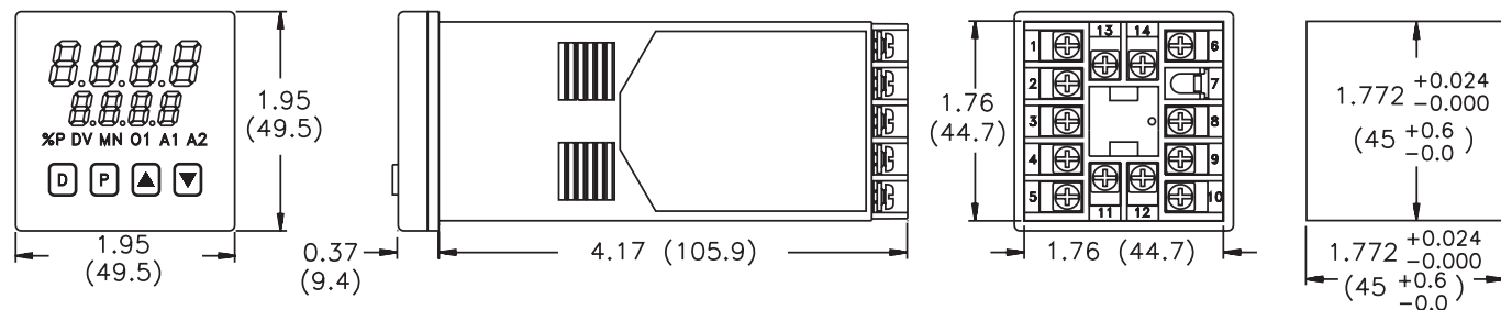
Figure 43, Dimensions
