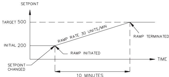
Figure 14, Setpoint Ramp Rate
