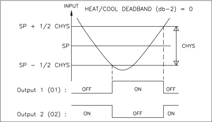
Figure 23, O1/O2 ON/OFF Control Software Revision V4.0 or Later
