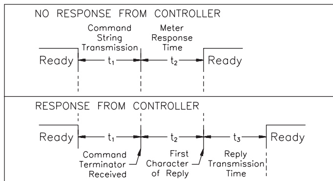
Figure 35, Timing Diagram
