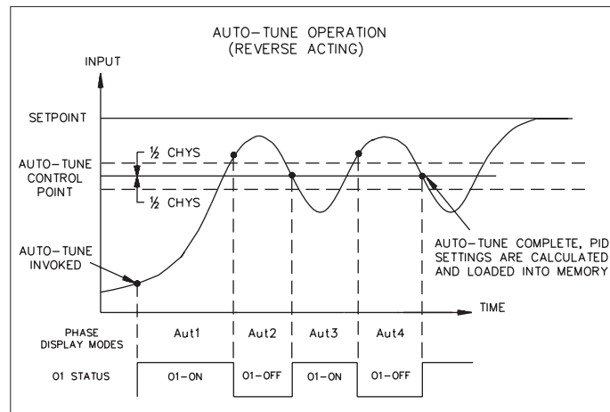
Figure 28, Auto-Tune Operation
