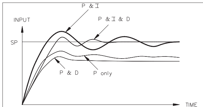
Figure 32, Typical Response Curve
