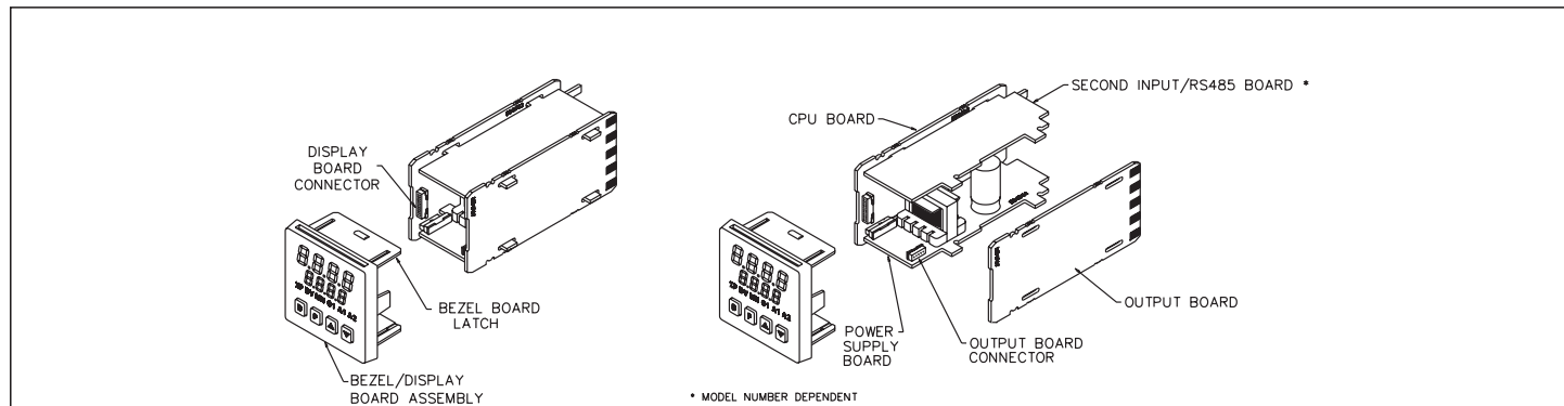
Figure 39, Output Board Replacement
