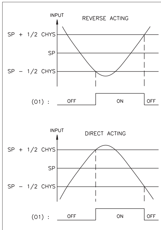
Figure 21, Output 1 (O1) ON/OFF Control Software Revision V4.0 or Later
