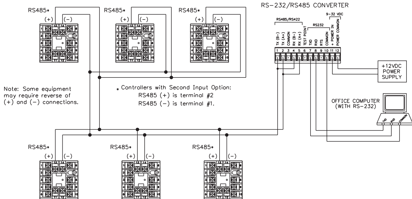
Figure 9, Connecting to a Host Terminal
