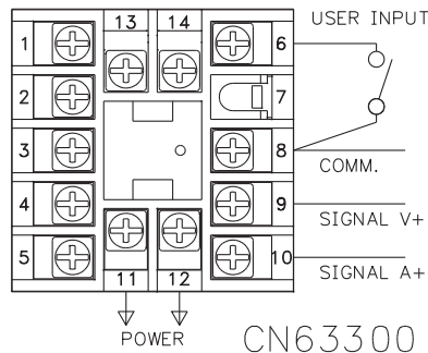
Figure 6, CN63300 Signal Connection
