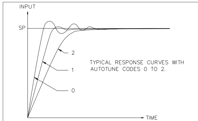
Figure 27, Auto-Tune Code
