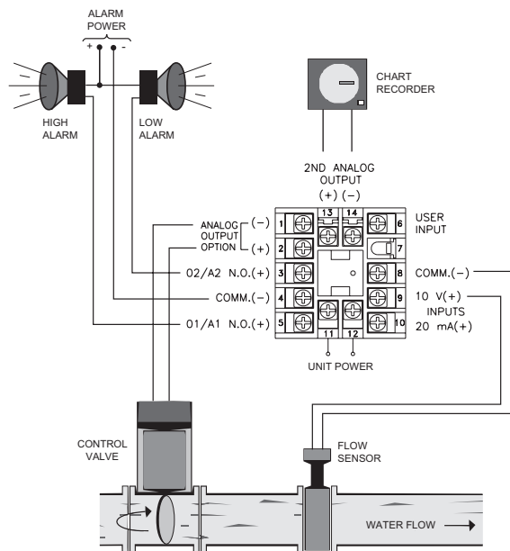
Figure 38, Water Processing Application
