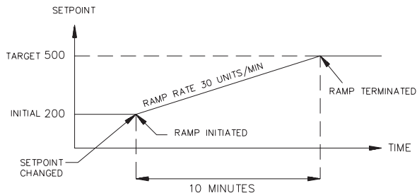
Figure 12, Setpoint Ramp Rate
