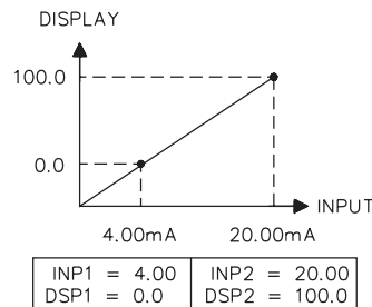
Figure 13, Scaling Points
