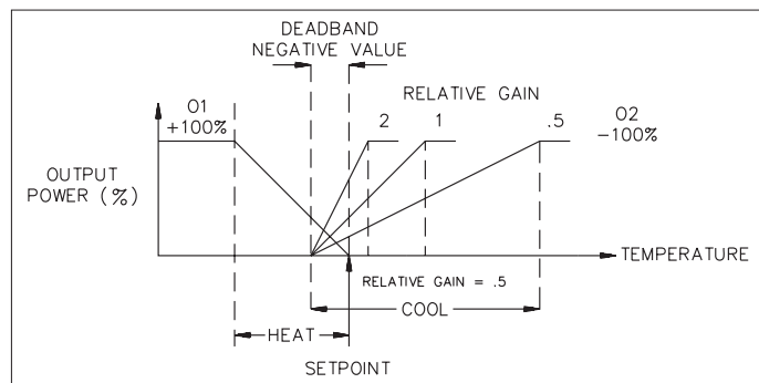
Figure 20, Heat/Cool Operation (db<0)
