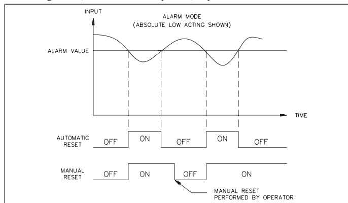
Figure 16, Alarm Reset Sequence
