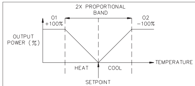
Figure 18, Heat/Cool Operation (db=0)
