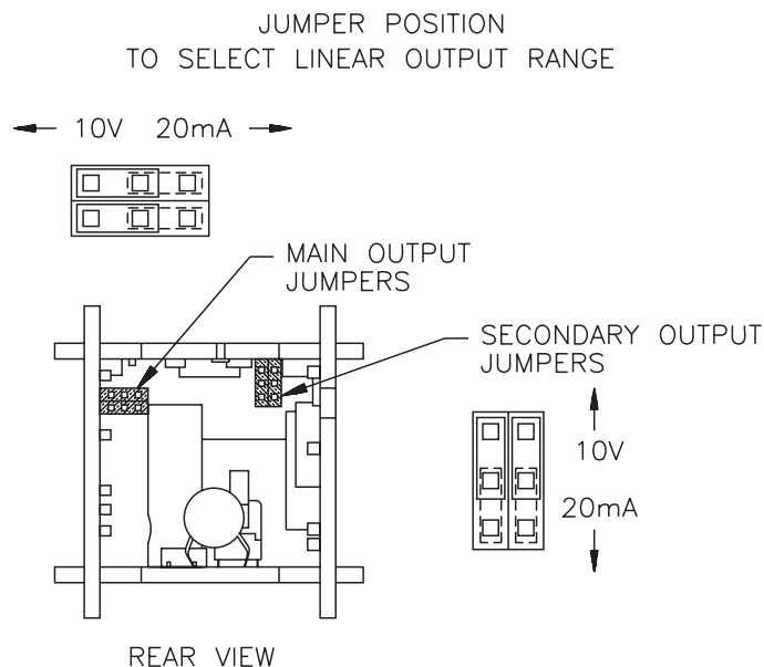
Figure 10, Linear Output Range Jumpers
