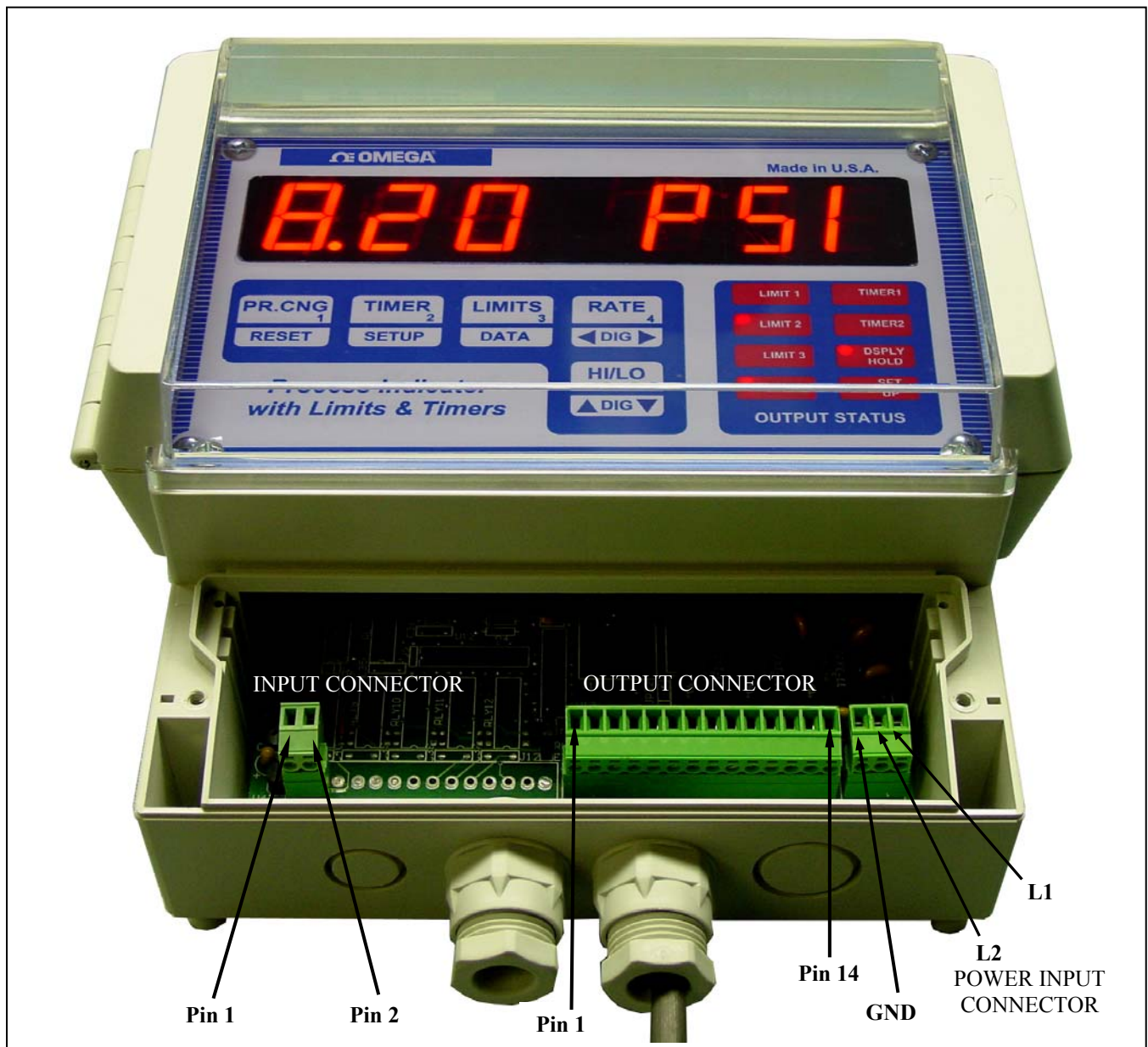
FIG- 3. DPS3311 Series TERMINAL COMPARTMENT
