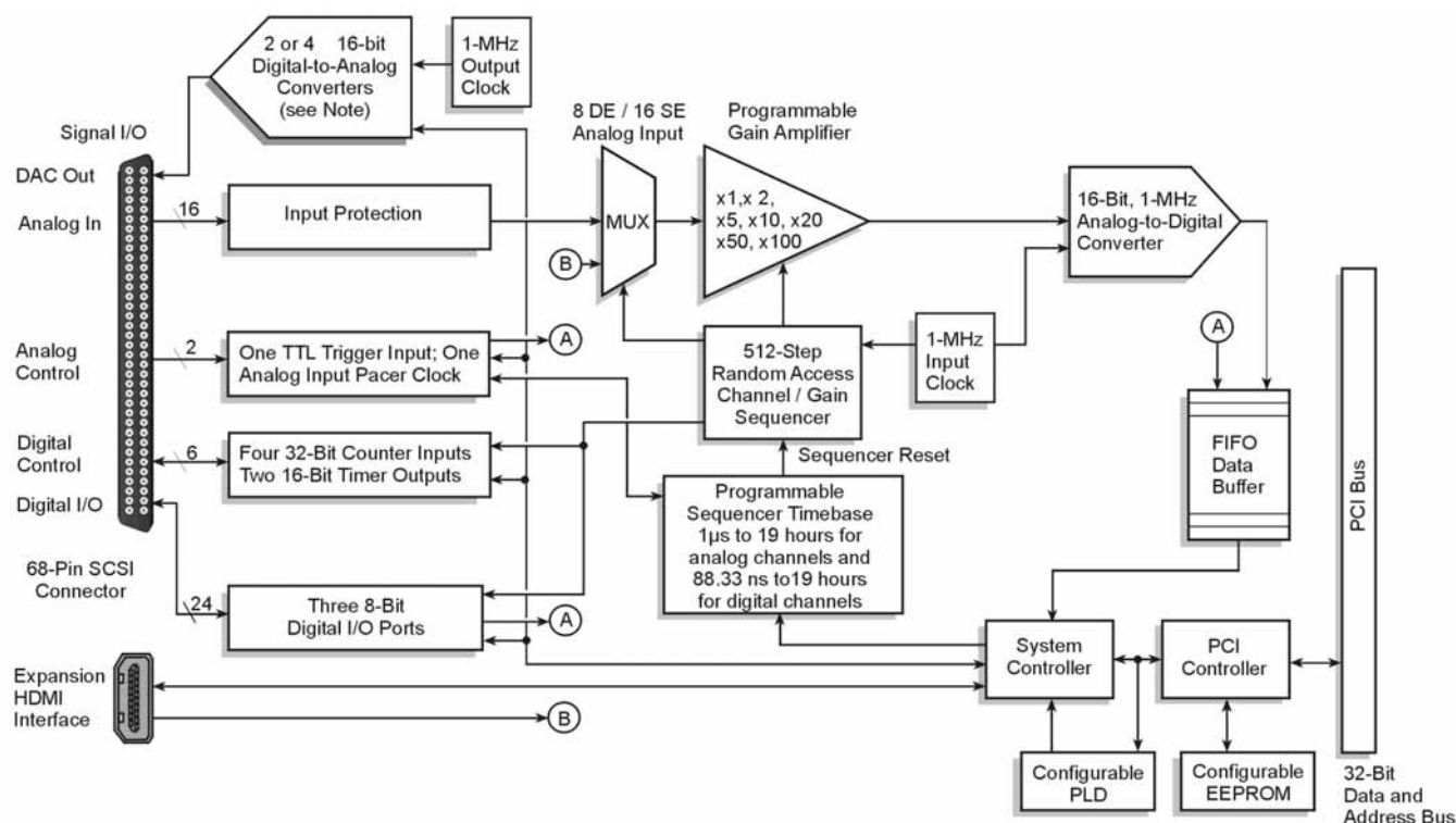
Block Diagram for DaqBoard/3000 and /3001
