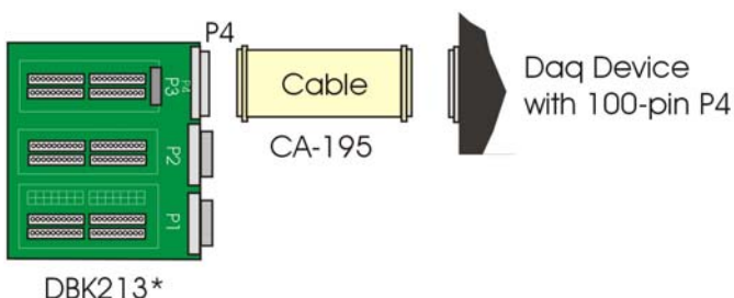
Connecting a DBK213
