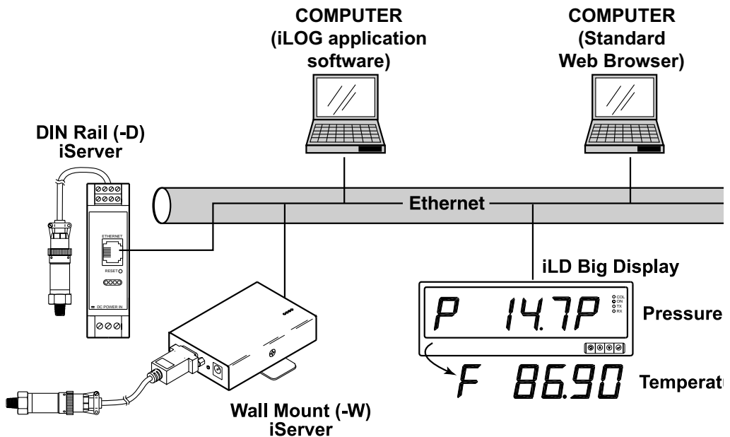
Figure 1.1 iServer with Probe on the Ethernet Network
