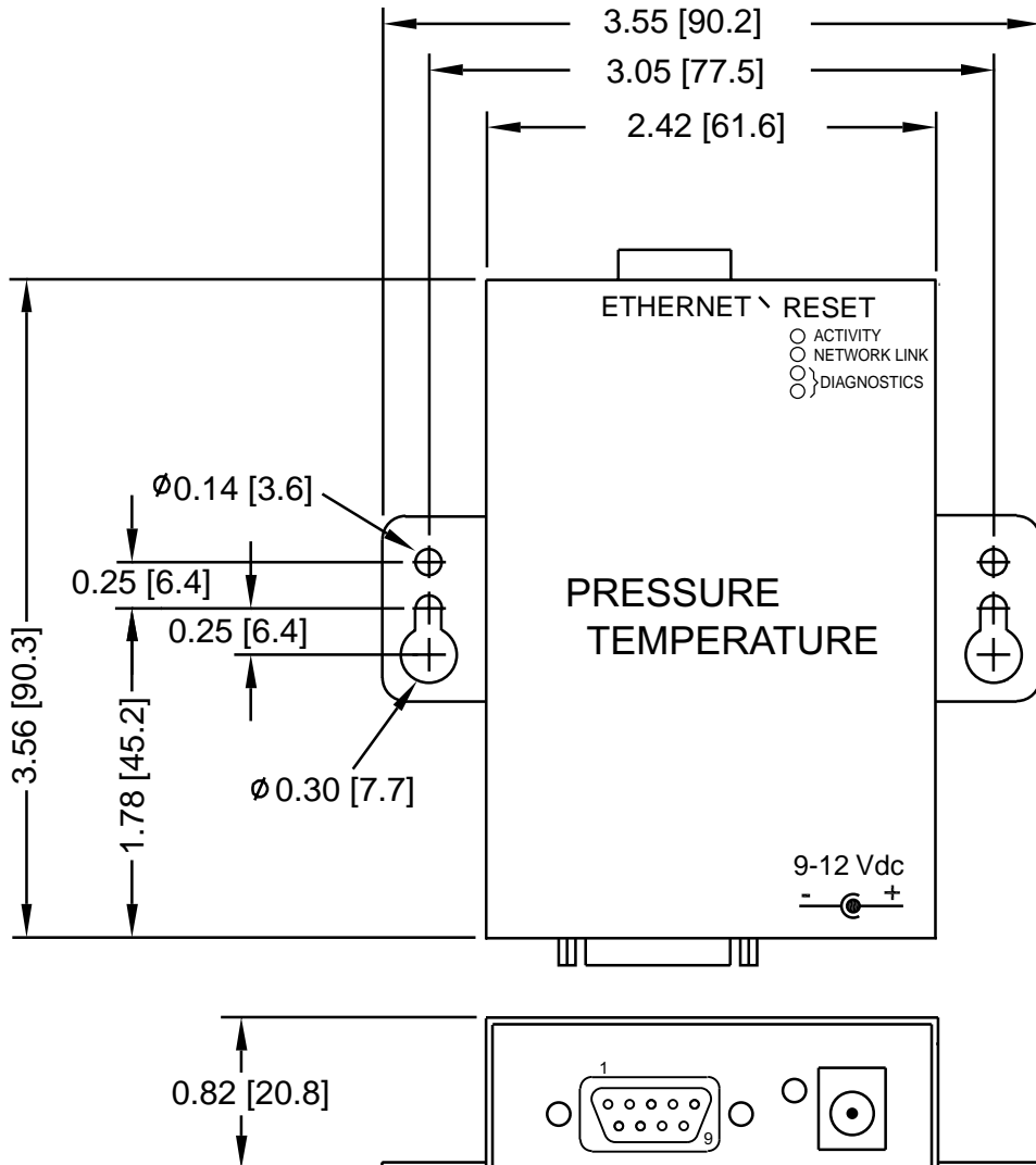
Figure 2.1 Mounting - Wall Mount iServer
