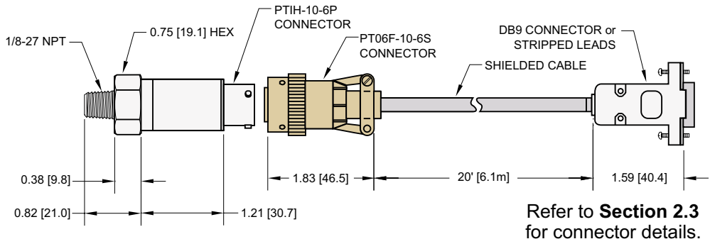
Figure 2.8 Probe Wiring Hookup
