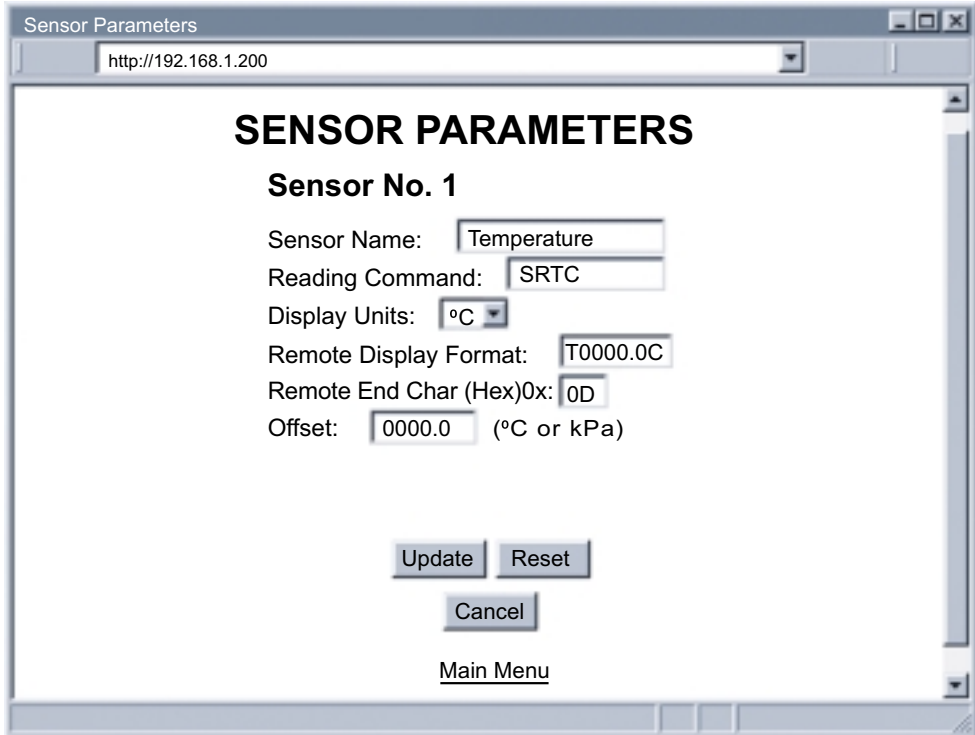
Figure 4.10 Sensor Parameters
