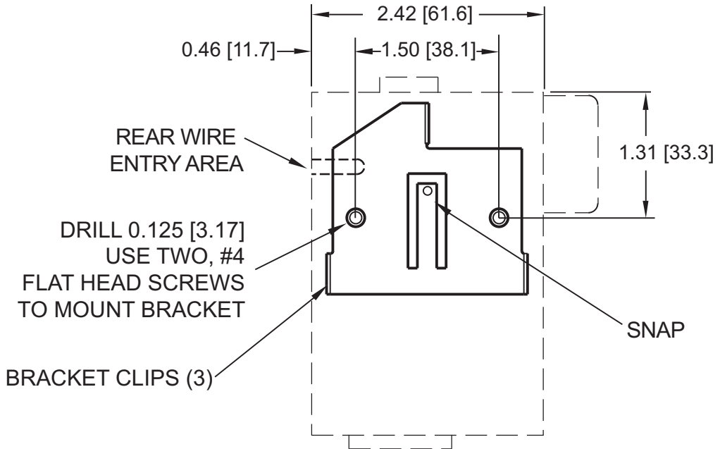
Figure 2.2 Wall Mounting
