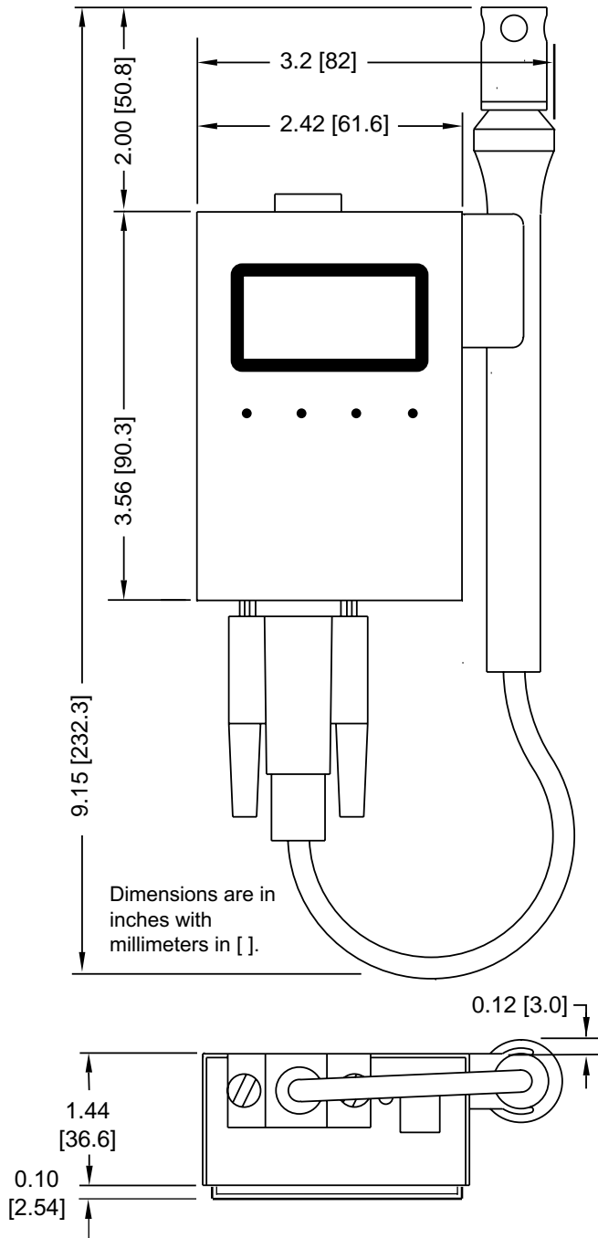
Figure 2.2 Dimensions
