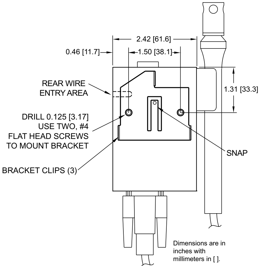
Figure 2.1 - Mounting Bracket
