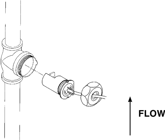
Figure 2-1. Horizontal Mounting Position
