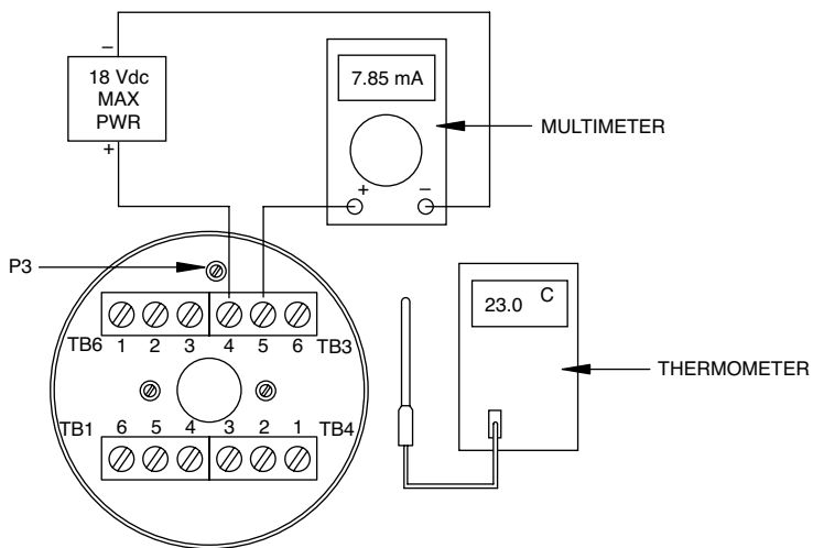
Figure 4-2. Temperature Calibration Setup
