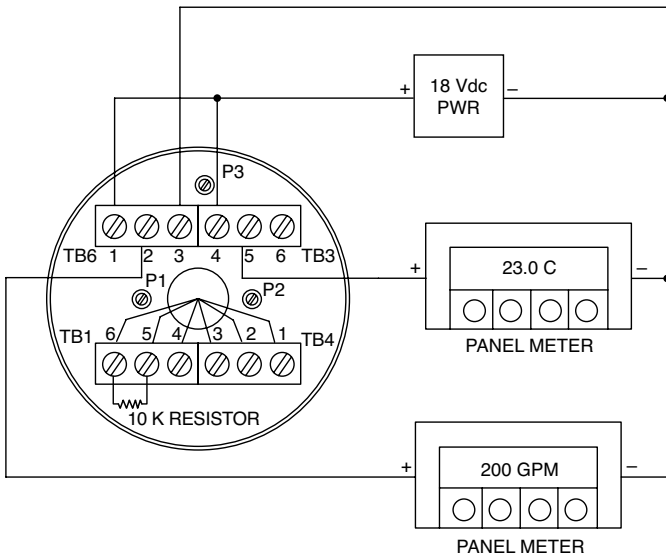
Figure 2-3. Basic Wiring Diagram
