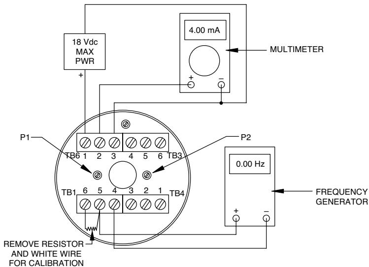
Figure 4-1. Flow Calibration Setup
