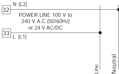
Fig. 18 POWER LINE WIRING
