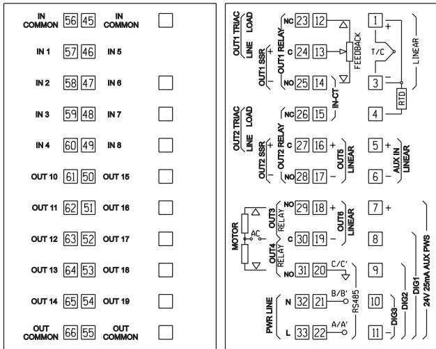
Fig. 3 REAR TERMINAL BLOCK
