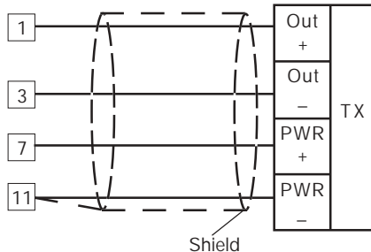
Fig. 7.C INPUTS WIRING FOR 4-WIRE TRANSMITTER
