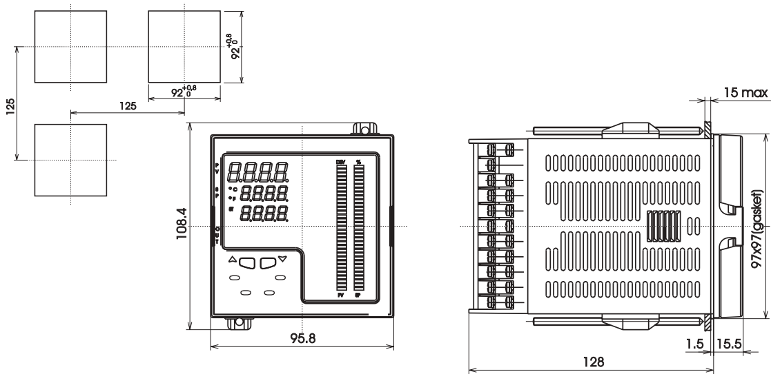
Fig. 2 OUTLINE AND CUT-OUT DIMENSIONS FOR MKP MODEL
