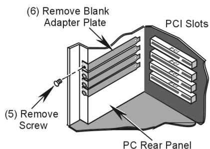
Removing a Blank Adapter Plate (Steps 5 and 6)
