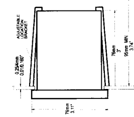
Side view of the panel-mounted unit
