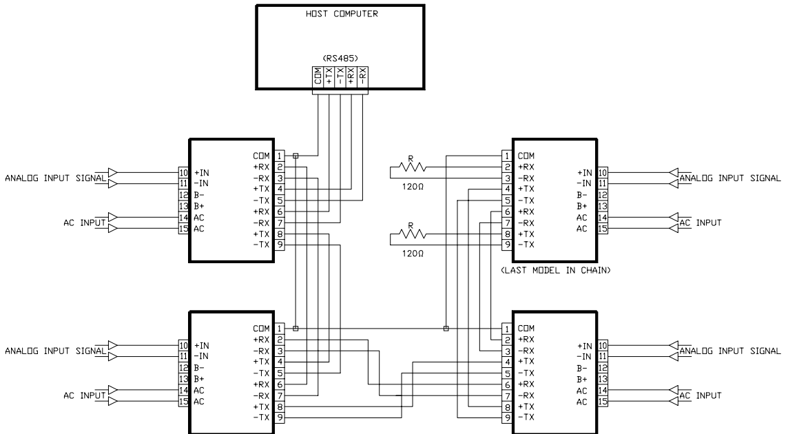
FIGURE 4. MULTIPLE UNIT RS485 COMMUNICATIONS SETUP
