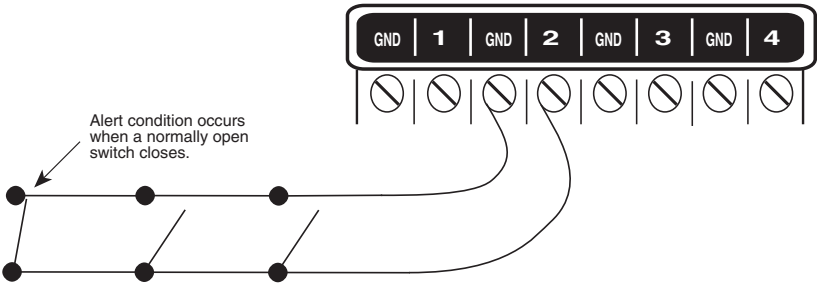
Figure 2-9. Multiple Normally Open Sensors
