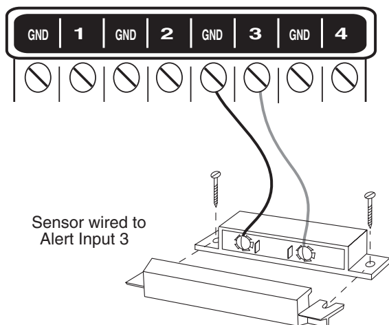
Figure 2-6. Sensor Connected to an Alert Input
