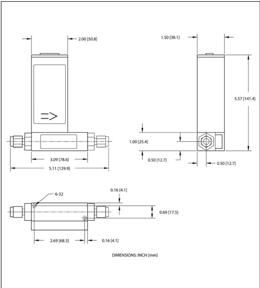
FMA 1500 FOR RANGES UP TO 10 L/MIN MASS FLOW METER
