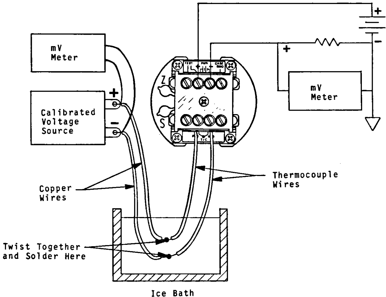
Figure 5-3 Calibration Setup
