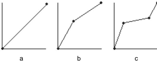
Figure 8. Breakpoint Examples
