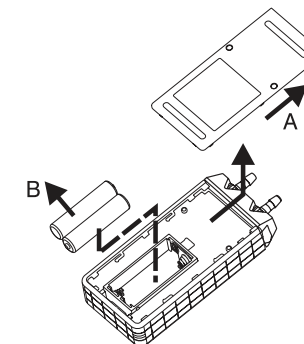
A. Battery Cover B. Battery
