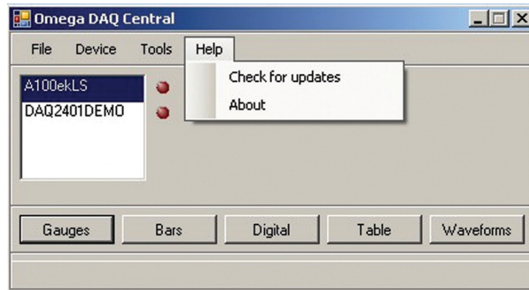
Figure 4-8. Help Menu
