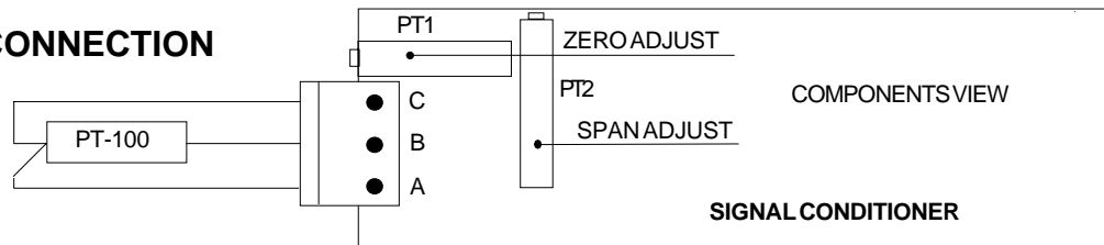
2 WIRE CONNECTION
