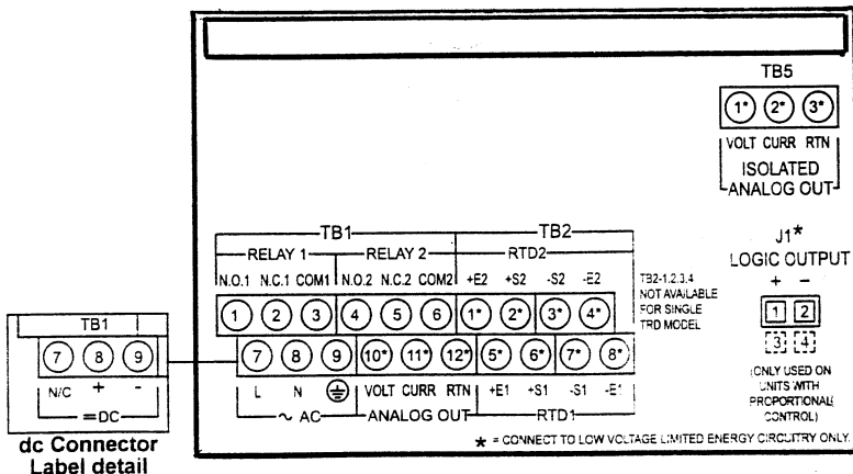
Figure 1.1 - Principaux raccordements
